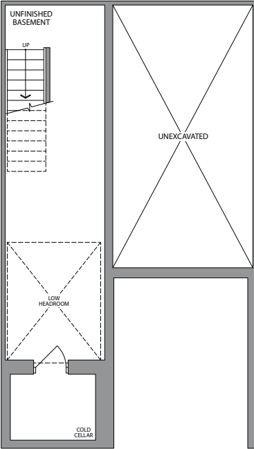
BASEMENT ELEVATION 1
