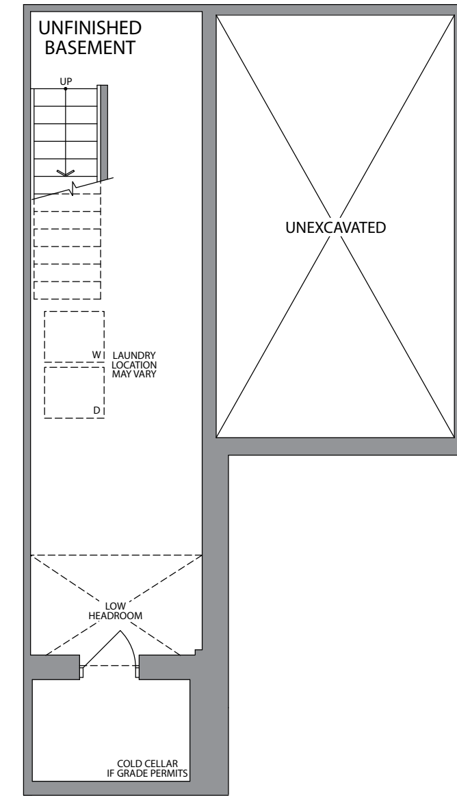
BASEMENT ELEVATION 1 & 2
