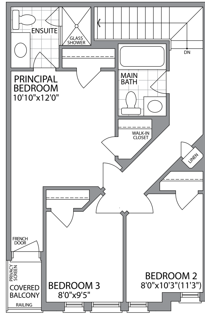
THIRD FLOOR ELEVATION 1
