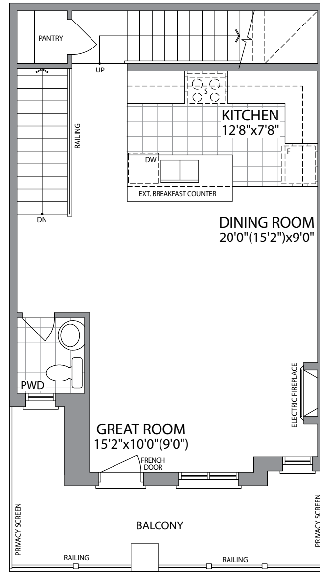
MAIN FLOOR ELEVATION 1
