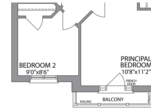
OPT. THIRD FLOOR W/4 BEDROOMS ELEVATION 2C
