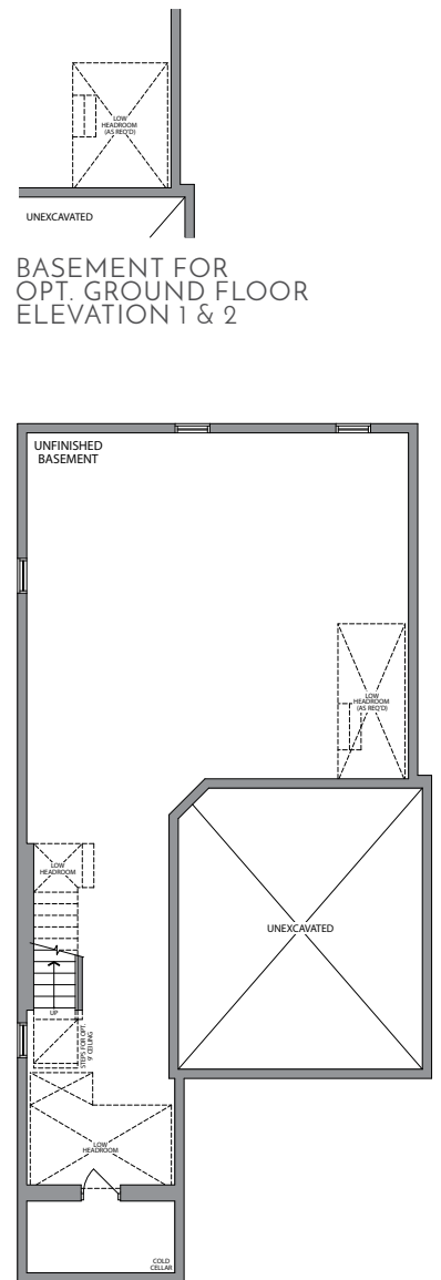
BASEMENT ELEVATION 1 & 2
