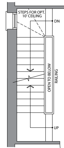
SECOND FLOOR FOR OPT. LOFT ELEVATION 1 & 2
