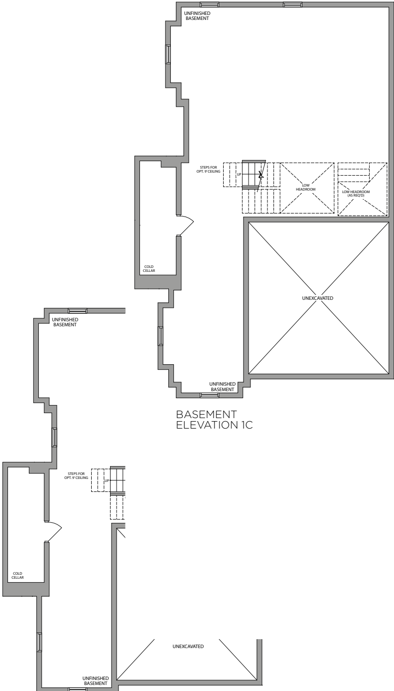
ELEVATION 1C
