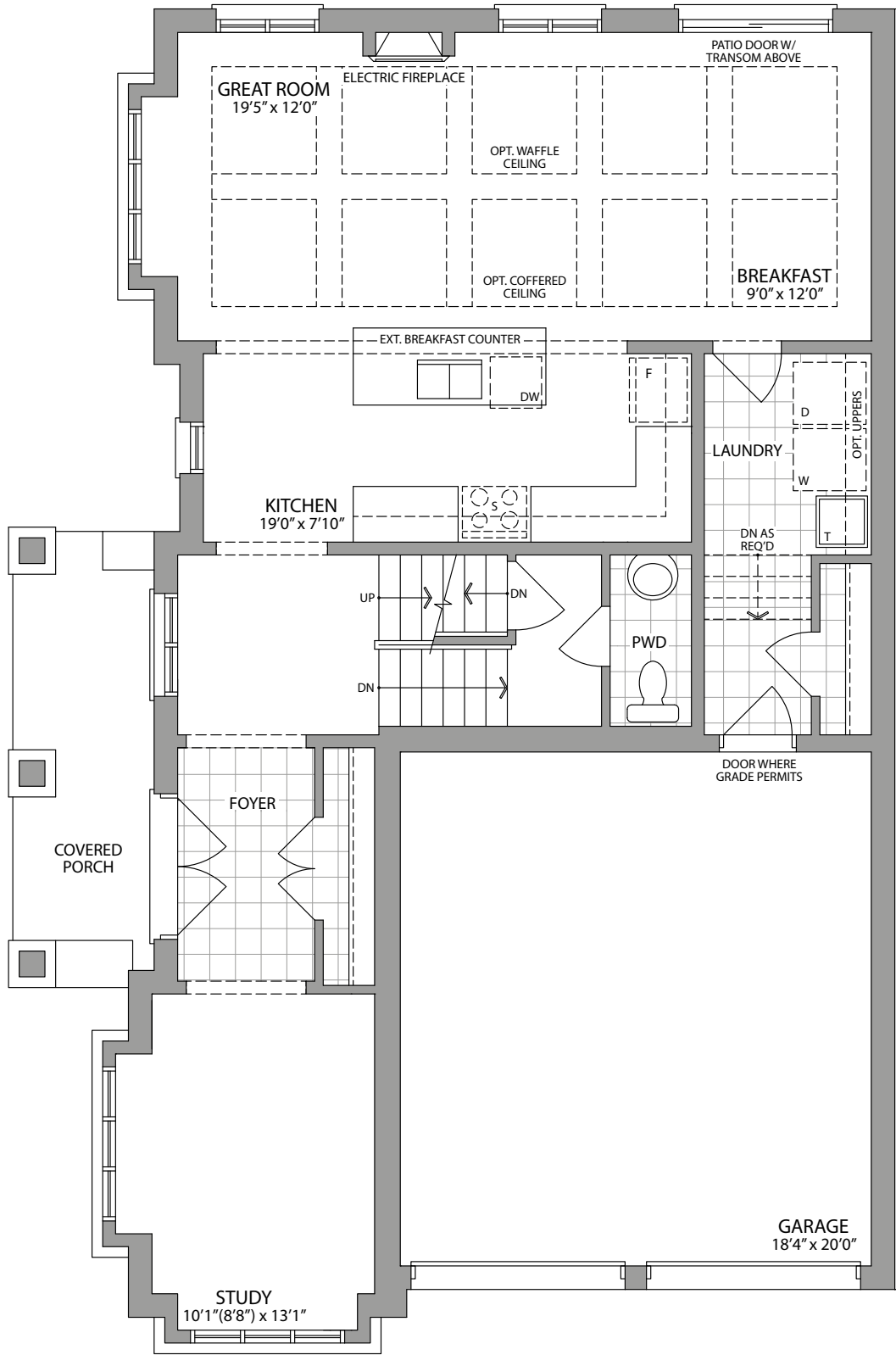
GROUND FLOOR ELEVATION 1C
