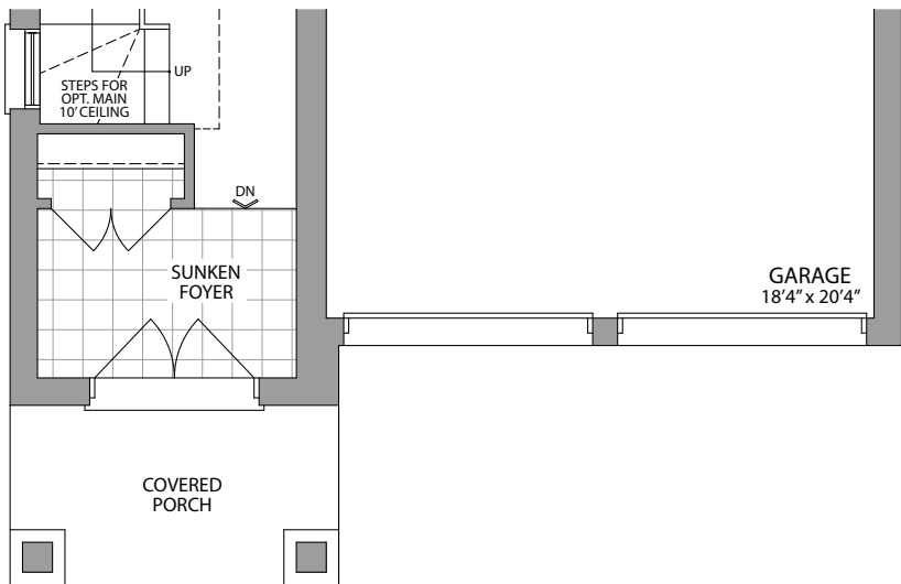
GROUND FLOOR ELEVATION 2
