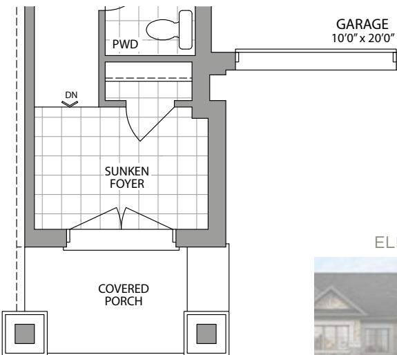
GROUND FLOOR ELEVATION 2/2C
