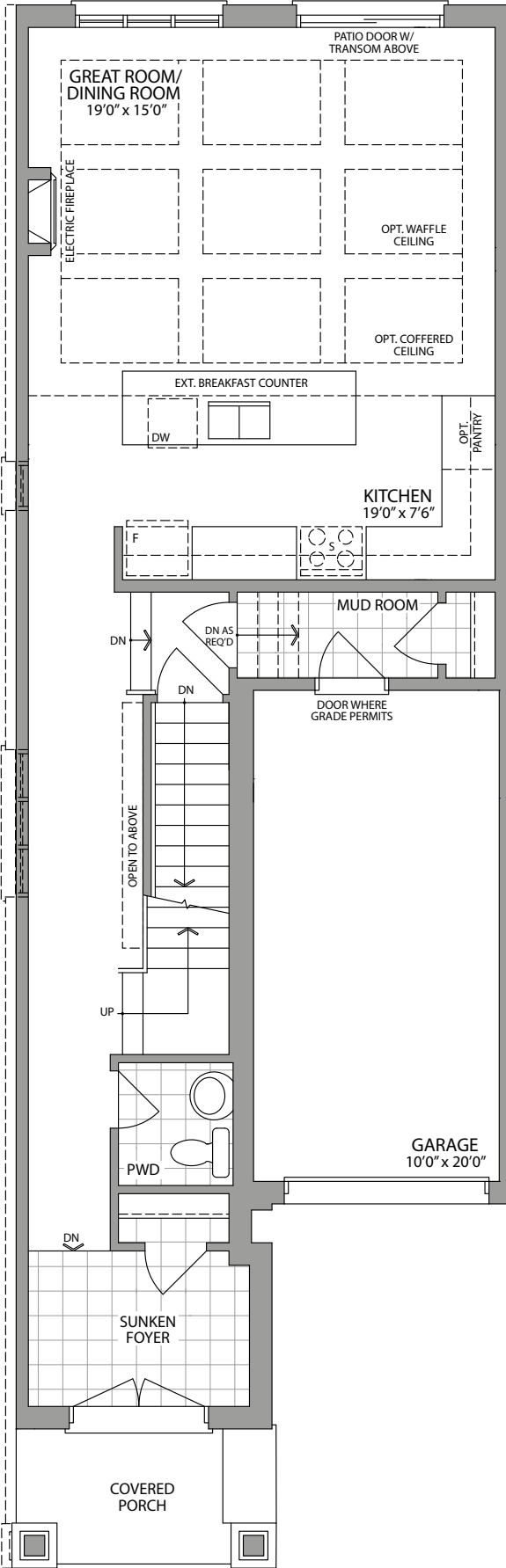
GROUND FLOOR ELEVATION 1/1C
