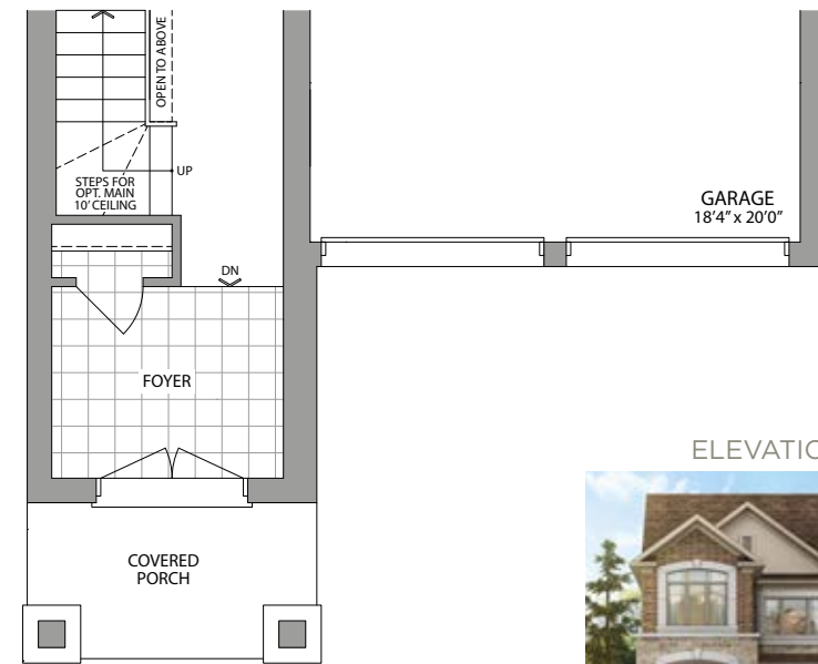
GROUND FLOOR ELEVATION 2
