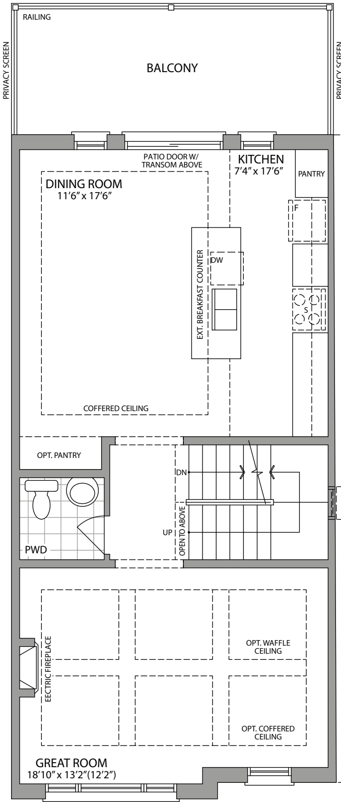
MAIN FLOOR ELEVATION 1/1C
