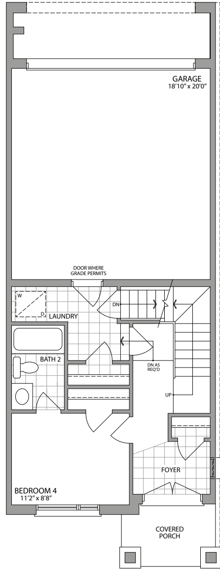
OPT. GROUND FLOOR W/4 BEDROOMS ELEVATION 1/1C
