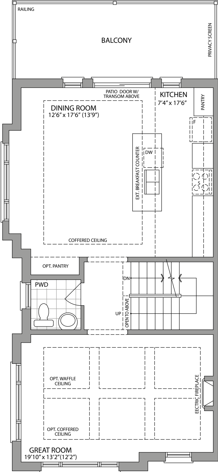
MAIN FLOOR ELEVATION 1C
