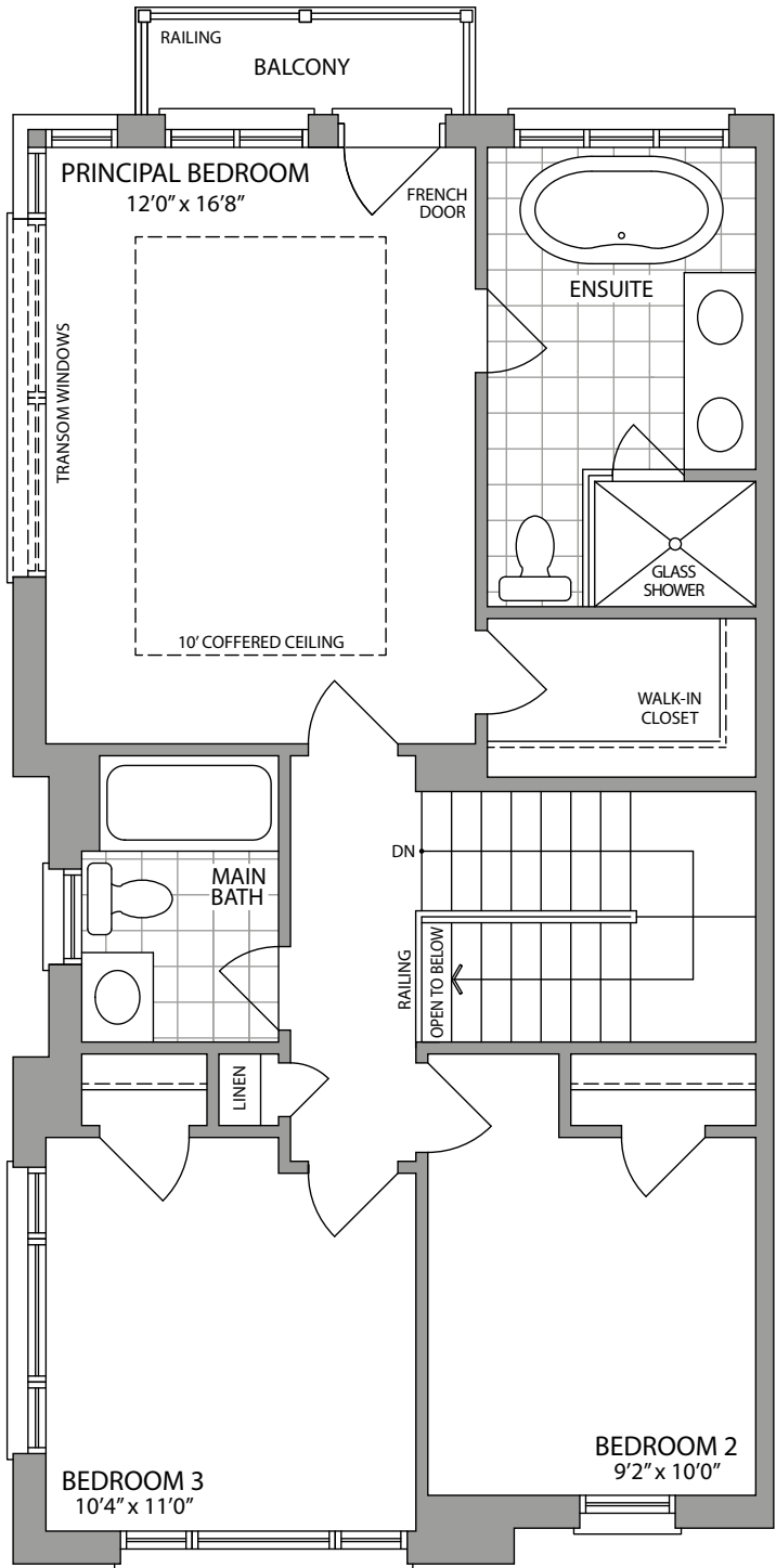
THIRD FLOOR ELEVATION 1C
